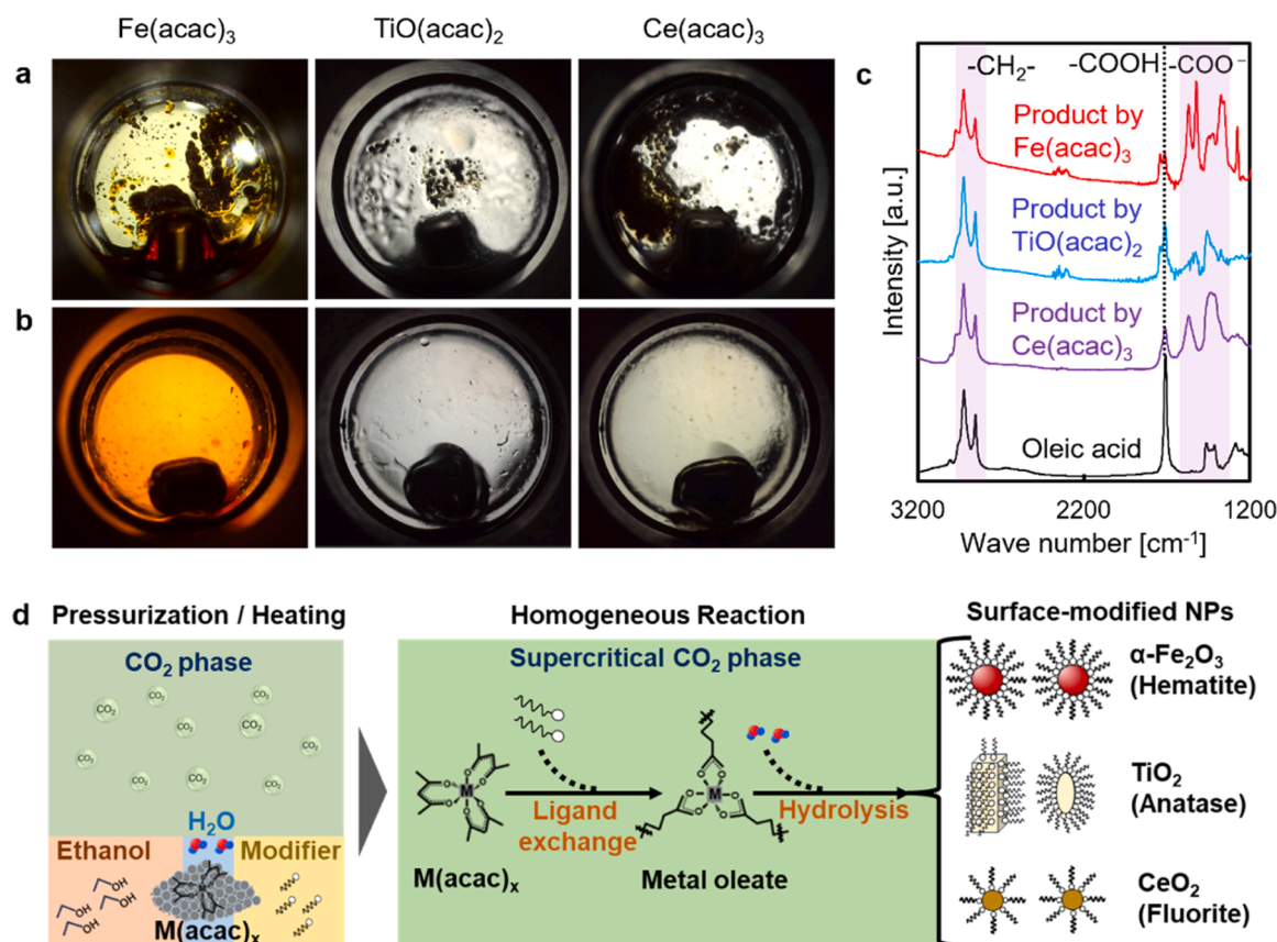
Fig. 4. Phase state (a) before pressurization/heating and (b) after pressurization/heating. (c) FT-IR spectra of products obtained without water addition and before post-treatment. (d) Proposed formation mechanism of various surface-modified NPs in scCO 2 atmosphere.
