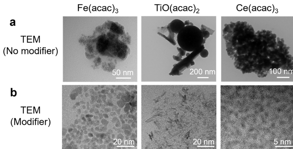
Fig. 1. TEM images of products synthesized (a) without surface modifier and (b) with surface modifier for Fe(acac)_3 , TiO(acac)_2 , and Ce(acac)_3 precursors.
