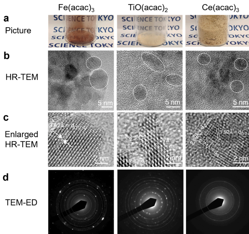
Fig. 2. Characterization results of products synthesized with surface modifiers for \text{Fe}(\text{acac})_3 , \text{TiO}(\text{acac})_2 , and \text{Ce}(\text{acac})_3 precursors. (a) Photographs, (b) HR-TEM images, (c) magnified HR-TEM images, and (d) TEM-ED patterns.
