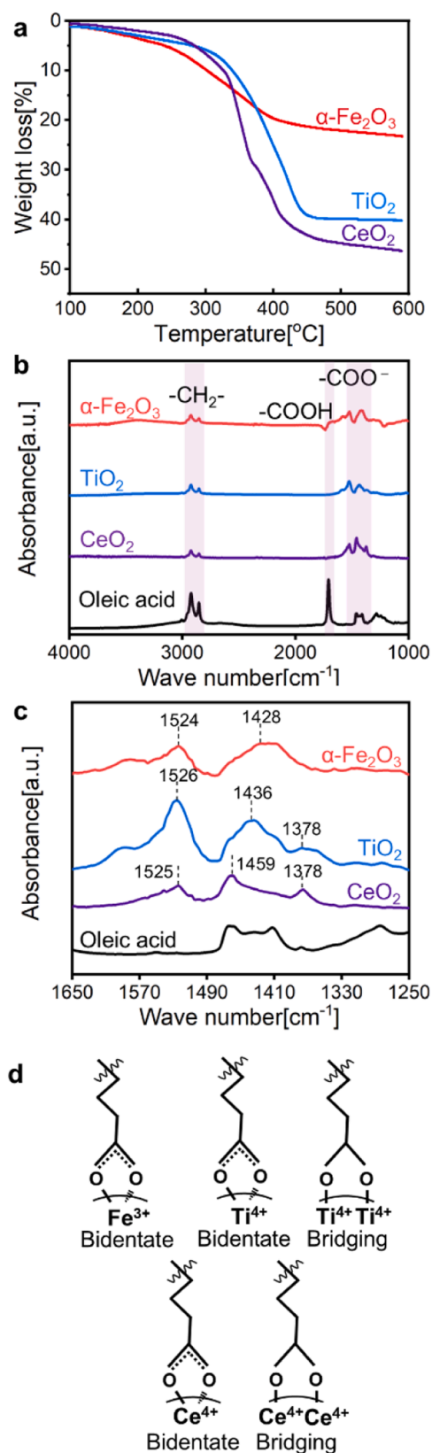
Fig. 3. Characterization results and estimated surface illustration of \alpha\text{-Fe}_2\text{O}_3 , \text{TiO}_2 , and \text{CeO}_2 NPs synthesized with surface modifier. (a) TG curves, (b) FT-IR spectra, (c) magnified FT-IR spectra, and (d) estimated surface states.
